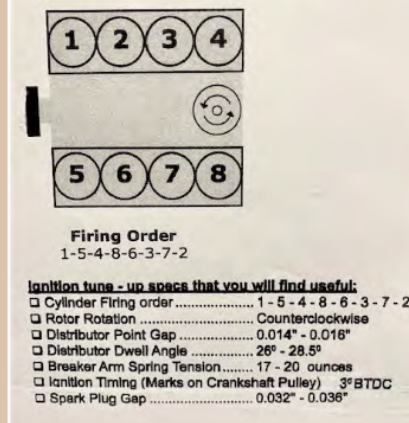
Fig. 2 – An example of timing and wiring information. This is typically avail from the manufacturer or on the internet.
