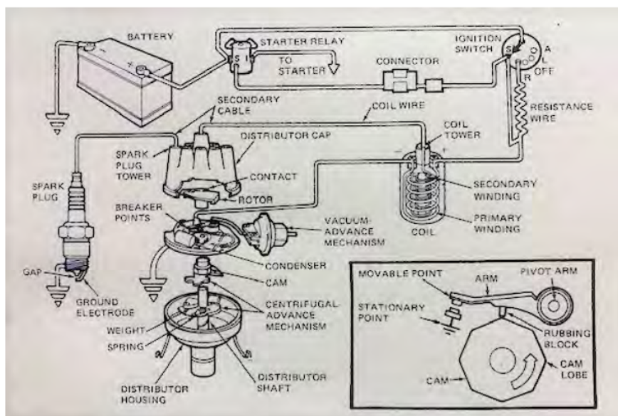
Fig. 3 – Schematic showing the ignition system components. Courtesy of Ford Motor Co.
